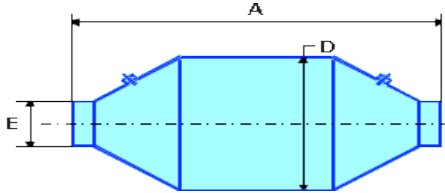
WELDED DESIGN
