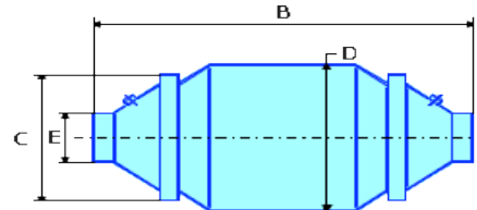
FLANGED DESIGN
